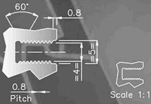
Detail of Screw (M5)
