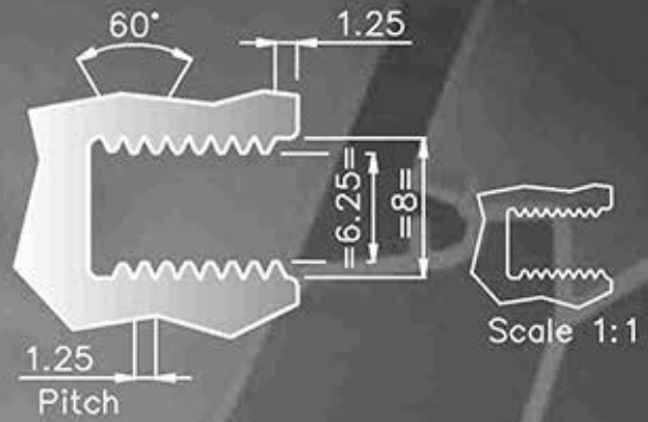
Detail of Screw (M8)
